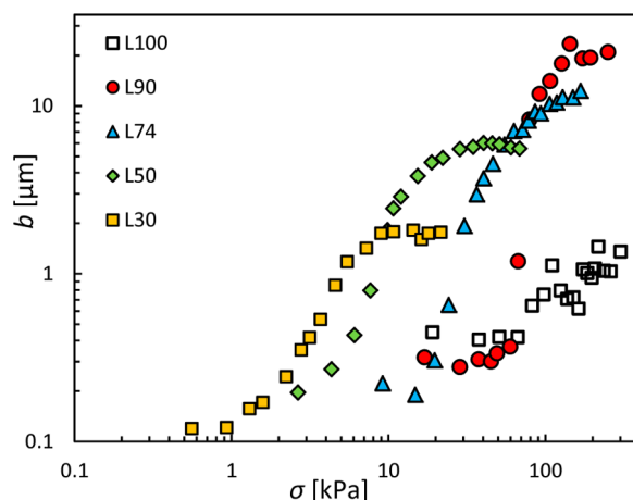
Figure 9. Slip length of binary 195K/4K PBDs versus shear stress.
