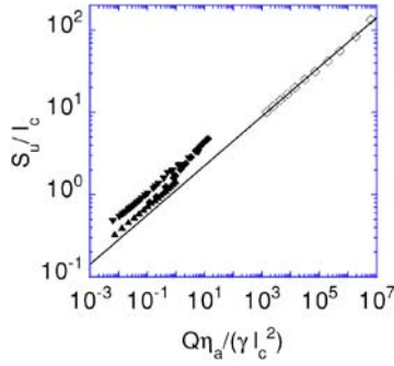
FIG. 7. Plot of the experimentally measured S_u/\ell_c versus (Q\eta_a)/(\gamma\ell_c^2) curves along with the curve predicted by the simulations of Lister [25]. The closed symbols depict the experimental measurements for systems 4, 6, and 7 in Table I, while the open symbols depict the range of (Q\eta_a)/(\gamma\ell_c^2) over which the simulations are performed. The solid line represents a power-law fit to the simulation results and has a slope of 0.30.
