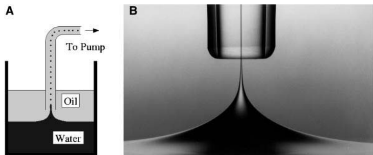
Fig. 1. (A) Diagram of the apparatus used in selective withdrawal. The tube orifice is a distance S from the unperturbed interface, and the rate of total fluid withdrawal is Q . A gear pump (Tuthill D9005M) was used to withdraw the fluids through a tube with S between 6.5 and 8.0 mm. Q was typically between 0.7 and 1.5 ml/s. Siphoning can also be used. (B) Photograph of a water spout entrained with the heavy mineral oil in a tube with orifice diameter 1.6 mm. The viscosities of the water and oil are 1.0 cSt and 195 cSt, respectively, at room temperature. The surface tension of the water-oil interface is 35 \pm 3 dynes/cm.
